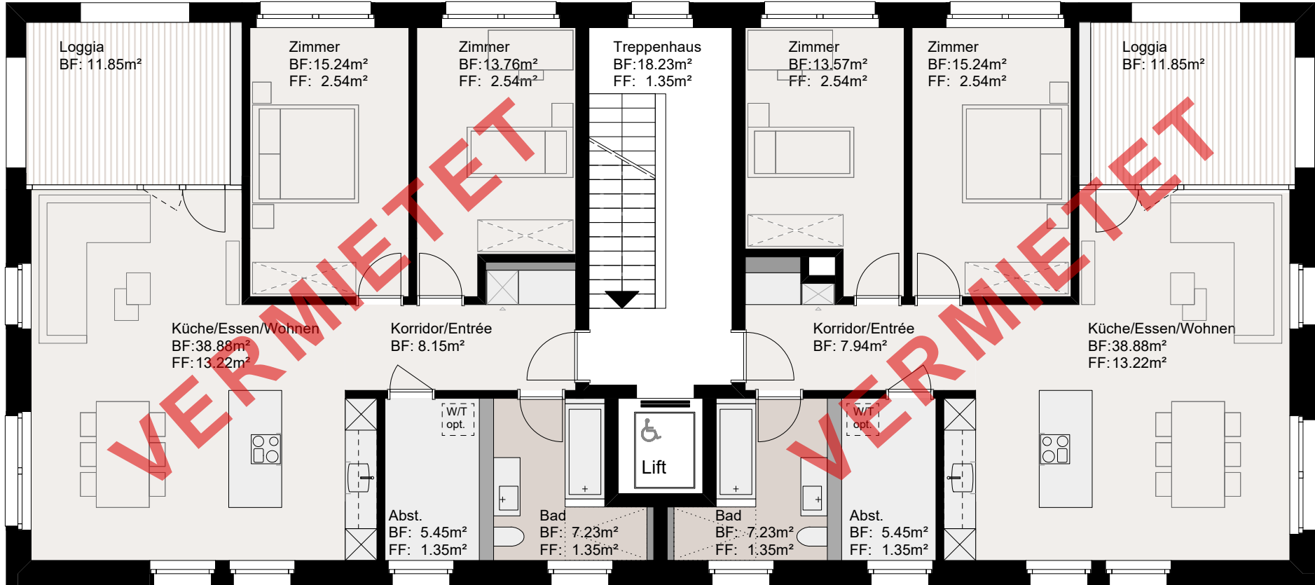
WHG A2.1 3.5-Zimmer NWF: 88.7m²
